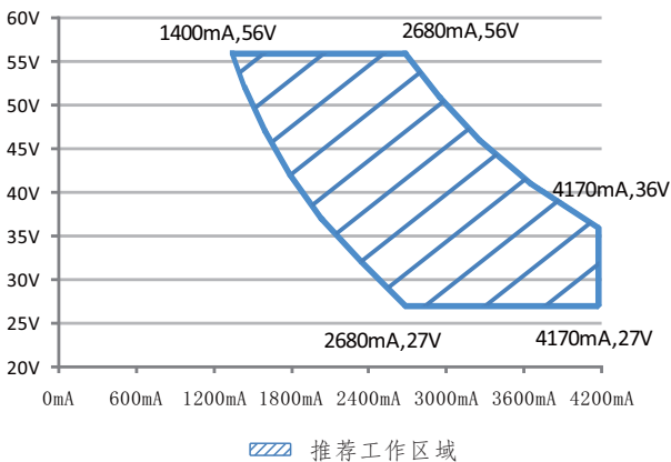
◎ XLG-150-H
